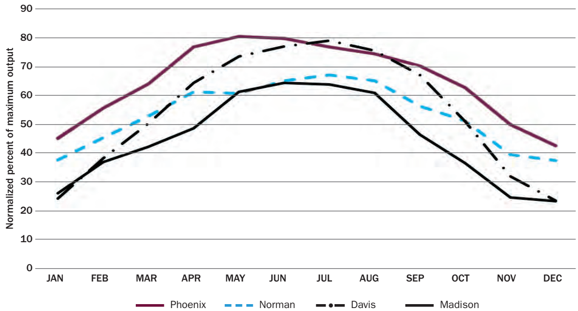
FIGURE 7 Monthly Solar Radiation for Four U.S. Locations
